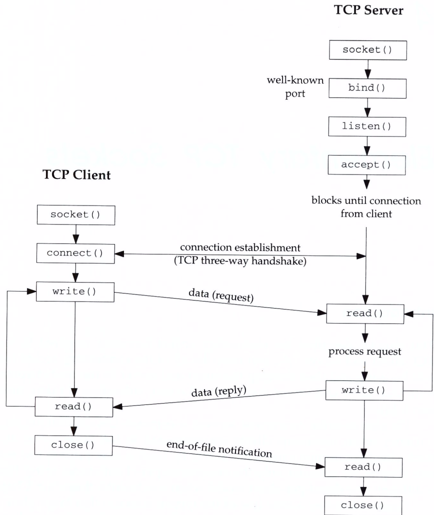
Figure 4.1 Socket functions for elementary TCP client-server.
