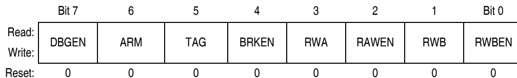
Figure 7-12. Debug Control Register (DBGC)
