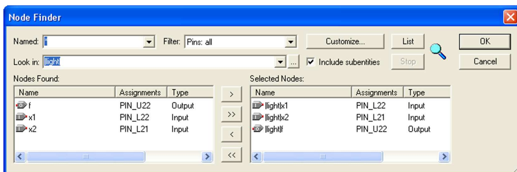
Figure 34. Selecting nodes to insert into the Waveform Editor.
