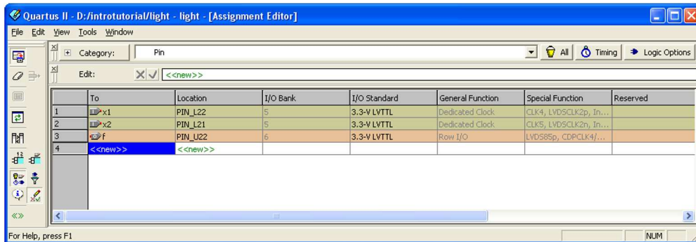
Figure 27. The complete assignment.
