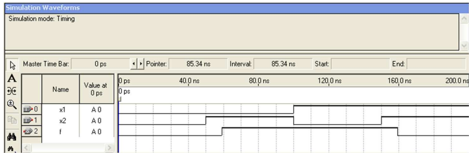
Figure 39. The result of timing simulation.
