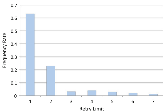
Fig. 5 Frequency of retr value usage
