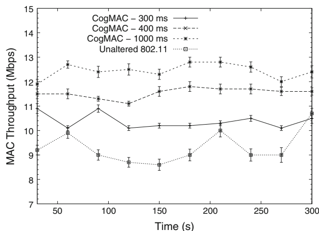
Fig. 15 Throughput with different access delay thresholds
