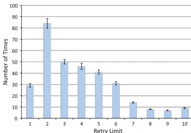
Fig. 11 Frequency of retry limit value usage with budget AD is 300 ms
