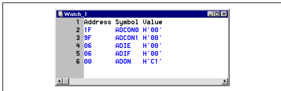
Figure 1.76: Watch Window
