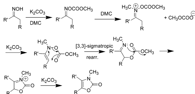
Scheme 11. Mechanism for the Synthesis of N -Methyl Oxazolinones from Oximes
