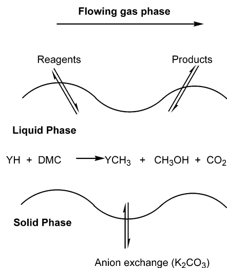
FIGURE 1. General mechanism of gas liquid-phase transfer catalysis (GL-PTC).
