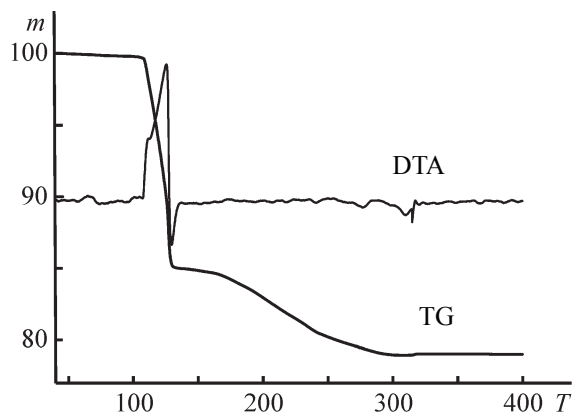
Fig. 2. Thermogram for salt (I) in hydrogen. ( m ) Sample mass (% of initial) and ( T ) temperature (°C); the same for Fig. 3
