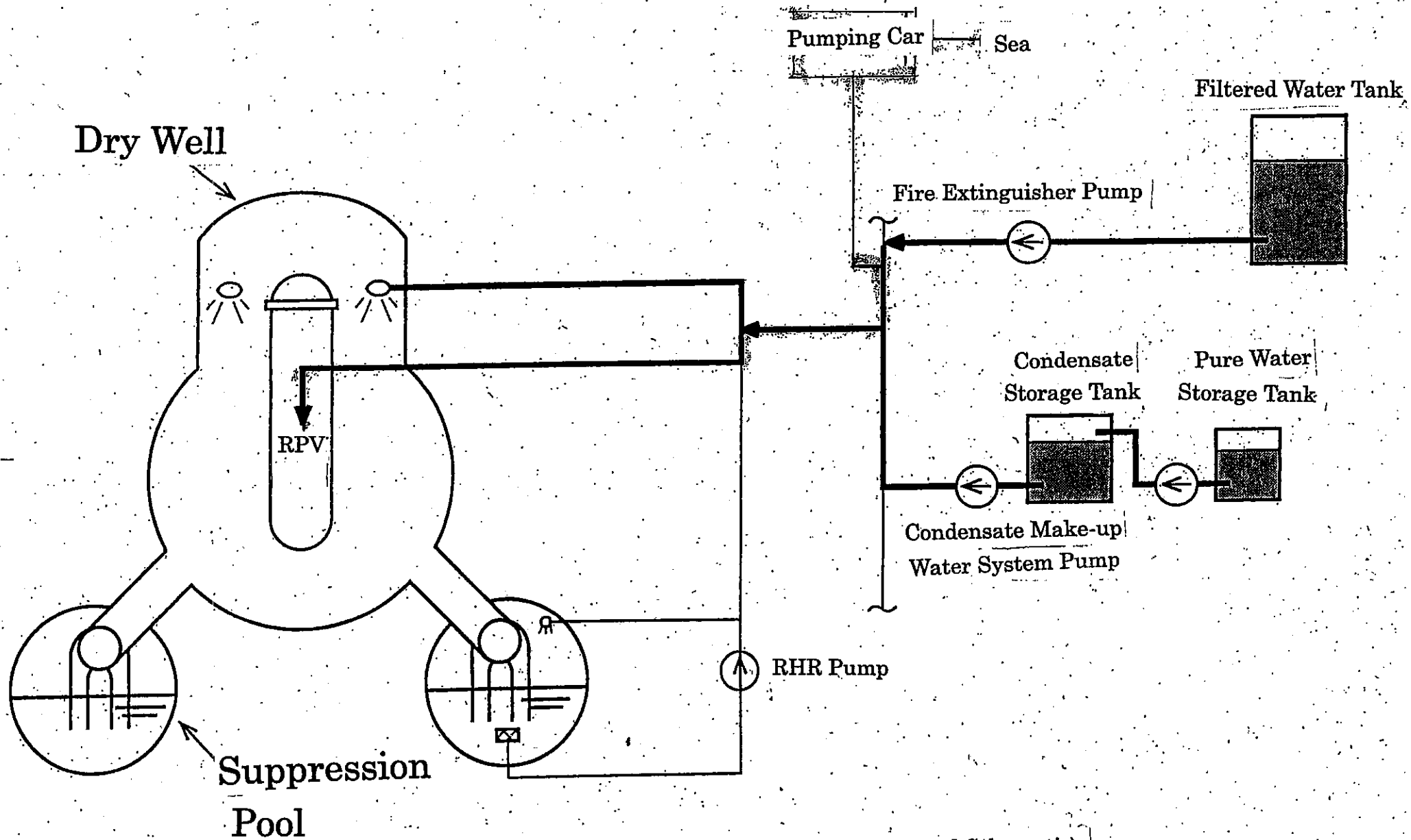
Alternate Water Injection System (Conceptual Schematic)
