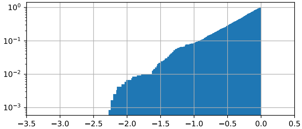
Histograma \log_{10}(F_i/\max\{F_{123}\}) 1794 MEPs cumulative (real) - mt 140
