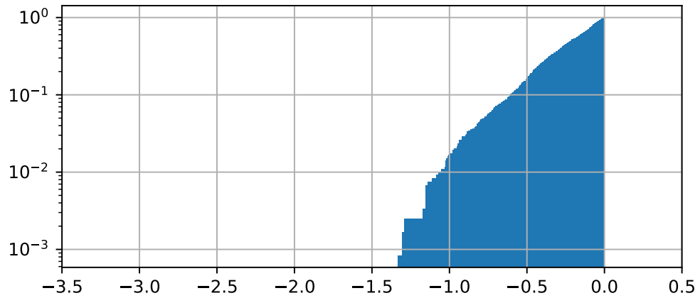
Histograma \log_{10}(F_i/\max\{F_{123}\}) 1797 MEPs cumulative (real) - mt 180
