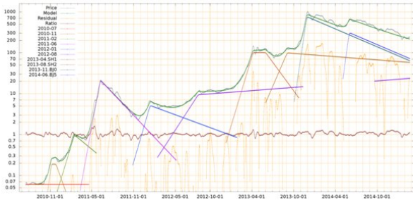
Price bubbles - 2010-06-20 to 2015-03-10 (smoothed with 15-day Hann window)
